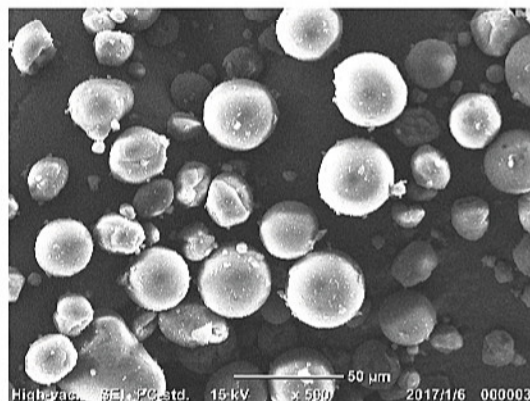
Scanning electron microscope (SEM) picture of omega powder, showing the advanced oil encapsulation technique.
